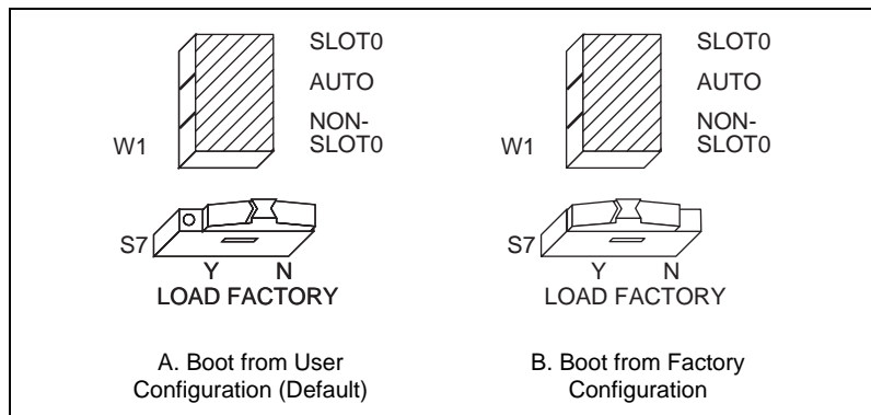
Figure C-3. EEPROM Operation
