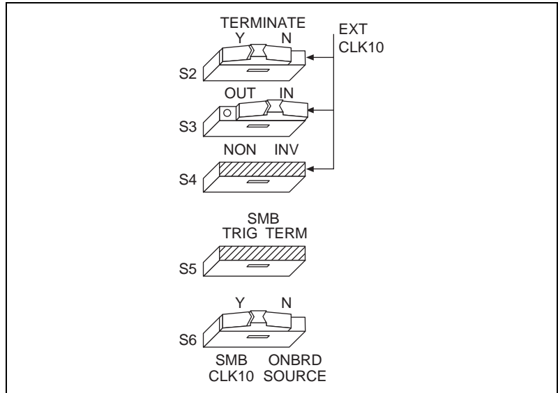
Figure C-7. Receive External CLK SMB with 50 \Omega Termination and Drive to the Backplane
