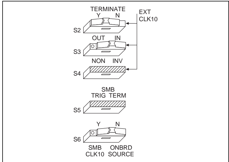
Figure C-5. Receive External CLK SMB with 50 Ω Termination
