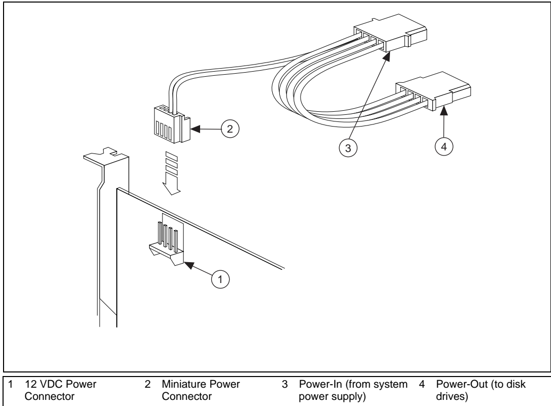
Figure 2-3. Connecting the Power Cable on the PCI-1394 host adapter
